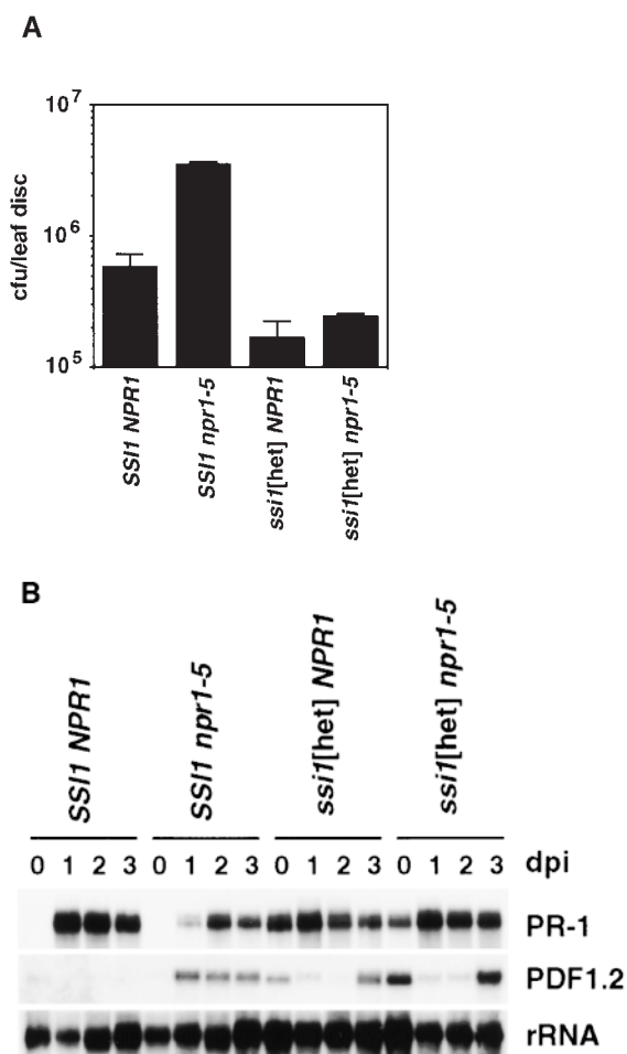
Figure 7. Growth of P. s. tomato DC3000 Containing the avrRpt2 Avirulence Gene and PR-1 and PDF1.2 Expression in Wild-Type ( SS11 NPR1 ), npr1-5 Mutant ( SS11 npr1-5 ), ssi1 Mutant ( ssi1[hel] NPR1 ), and ssi1 npr1-5 Double Mutant ( ssi1[hel] npr1-5 ) Plants.
