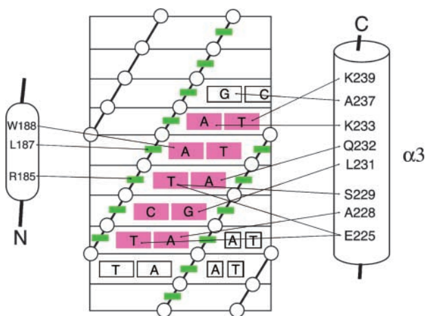
Figure 9. Scheme of the ARR10-B-DNA Interactions.
