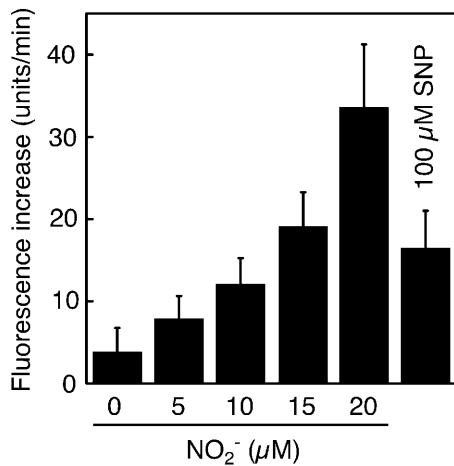
Figure 4. Nitrite-Dependent NO Production from Aleurone Layer Media.
