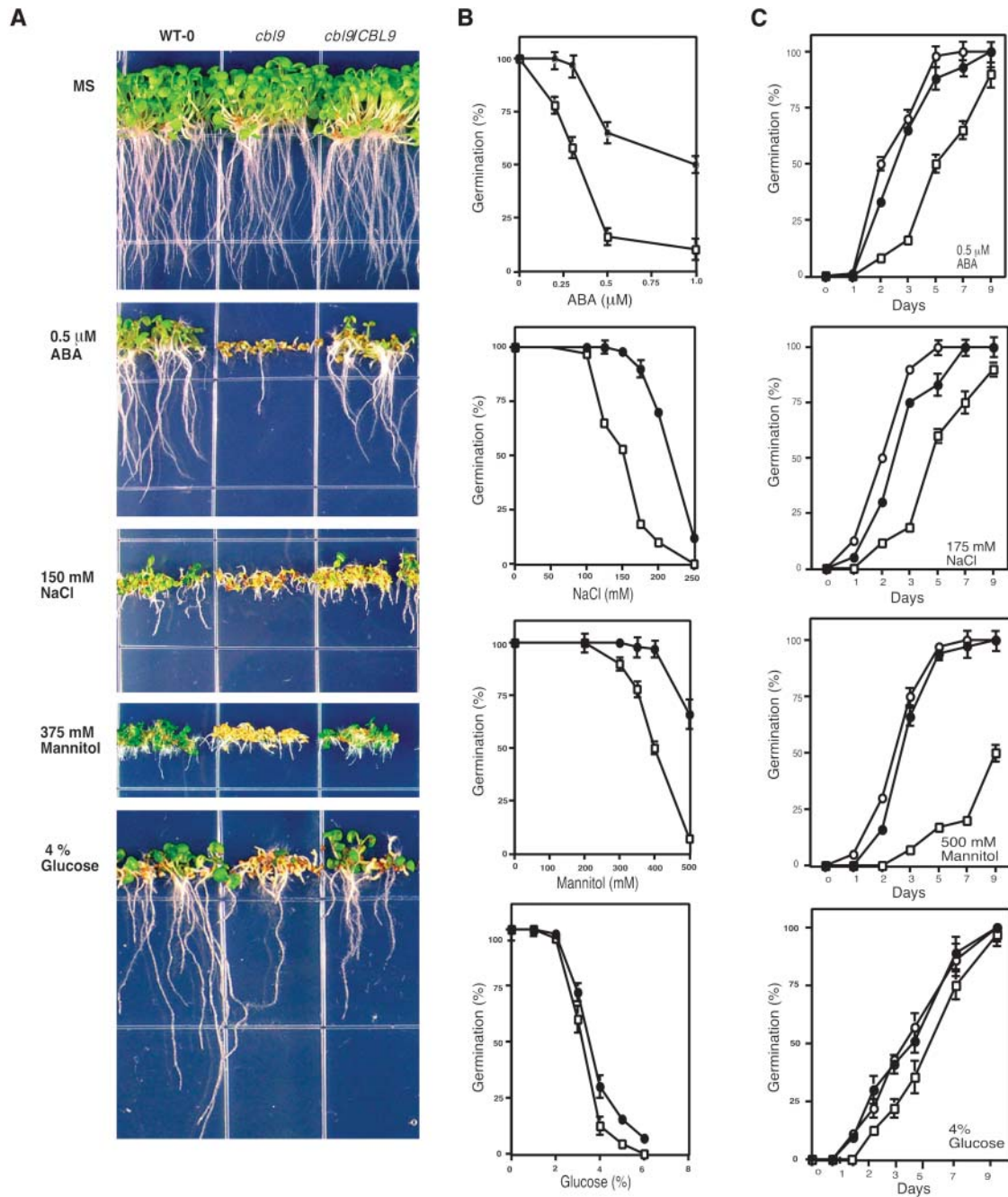
Figure 3. Germination of cbI9 Mutant Seeds Is Hypersensitive to ABA, Glucose, and Osmotic Stress Conditions.
